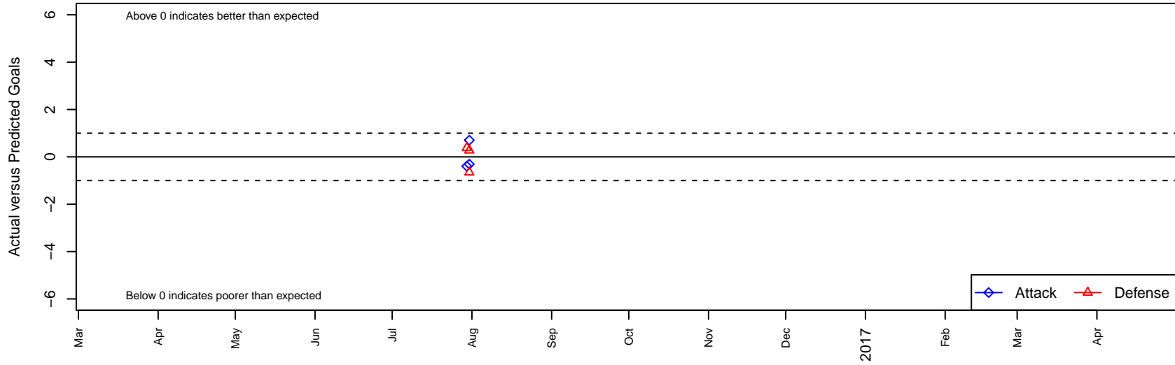
GPS National Team North G02 Dots are actual minus expected GF (blue circles) and GA (red triangles). Blue line is smoothed change in attack strength. Red is smoothed change in defense strength.
